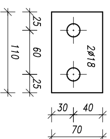
Poz.376, 4x, S355J2 Plate 10x70x110
