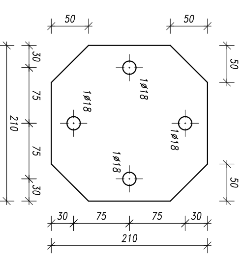
Poz.385, 24x, S355J2 Plate 12x210x210
