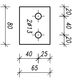
Poz.367, 28x, S355J2 Plate 8x65x80
