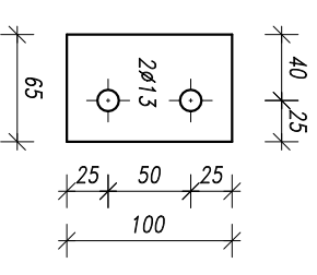
Poz.372, 44x, S355J2 Plate 8x100x65
