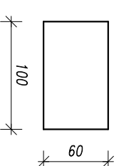
Poz.370, 14x, S355J2 Plate 8x60x100
