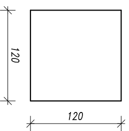
Poz.382, 24x, S355J2 Plate 12x120x120
