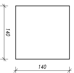
Poz.383, 14x, S355J2 Plate 12x140x140
