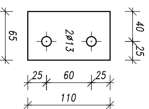
Poz.374, 224x, S355J2 Plate 8x110x65
