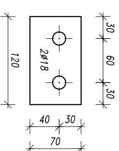
Poz.377, 28x, S355J2 Plate 10x70x120
