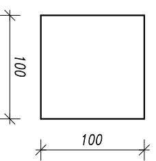
Poz.378, 14x, S355J2 Plate 10x100x100
