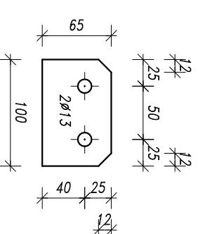
Poz.371, 48x, S355J2 Plate 8x65x100
