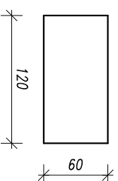
Poz.375, 24x, S355J2 Plate 8x120x60
