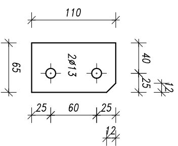
Poz.373, 24x, S355J2 Plate 8x110x65
