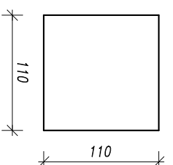
Poz.380, 196x, S355J2 Plate 10x110x110
