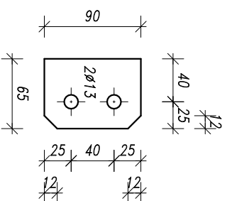
Poz.369, 272x, S355J2 Plate 8x90x65
