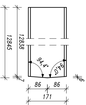
Poz.106, 2x HEA 180, S355J2
