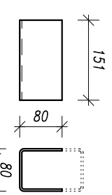
Poz.109, 6x RECT 120x80x4, S355J2H
