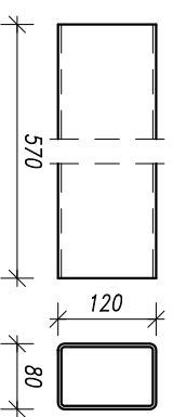
Poz.107, 4x RECT 120x80x4, S355J2H
