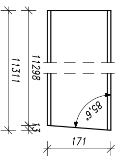
Poz.104, 2x HEA 180, S355J2
