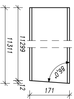
Poz.105, 2x HEA 180, S355J2
