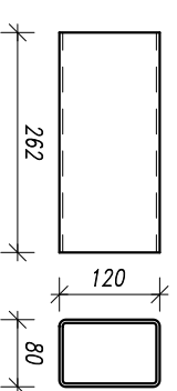
Poz.111, 4x RECT 120x80x4, S355J2H
