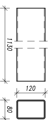
Poz.108, 2x RECT 120x80x4, S355J2H
