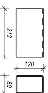
Poz.110, 4x RECT 120x80x4, S355J2H
