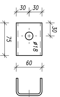
Poz.113, 8x, stal 1:5 C 60x40x4, S235JR
